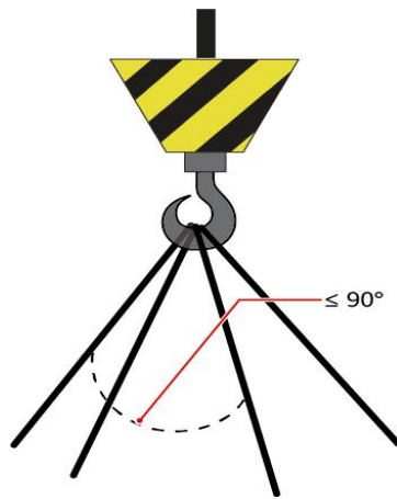
Figure 1-4 Cable angle requirements during lifting process
