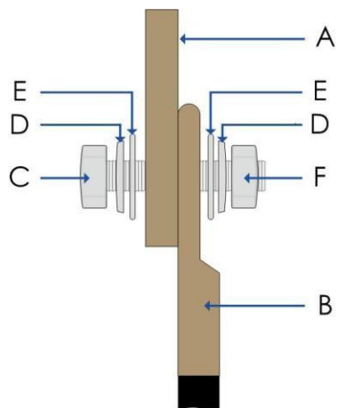
Figure 5.4 Copper terminal connection sequence
