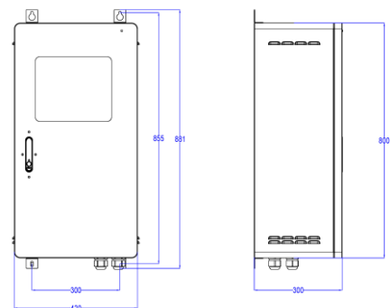
Fig. 3 – Product dimensions with HMI touch screen
